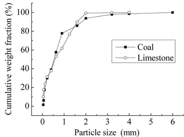
Fig. 2. Particle size distribution of the coal and limestone samples.
